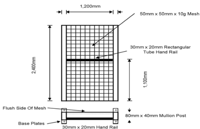
Mesh Partitioning With Hand Rail Fixed
