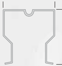
FRAME DETAIL
